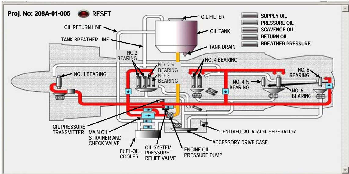
FIGURE A-17. Example of a system simulation.
